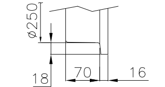
Wheel Profiles (For Reference)
